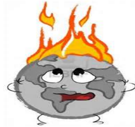
global warming
